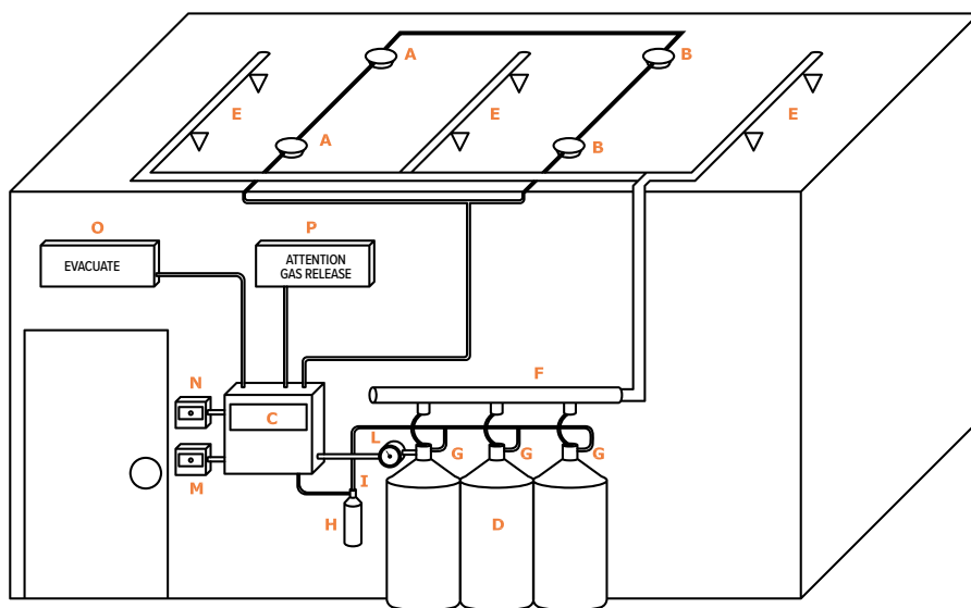
Application diagram
